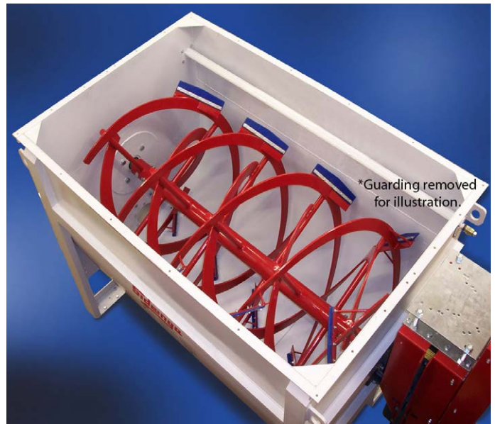
DOUBLE RIBBON MIXERS with capacities to 25 ton/hr.
